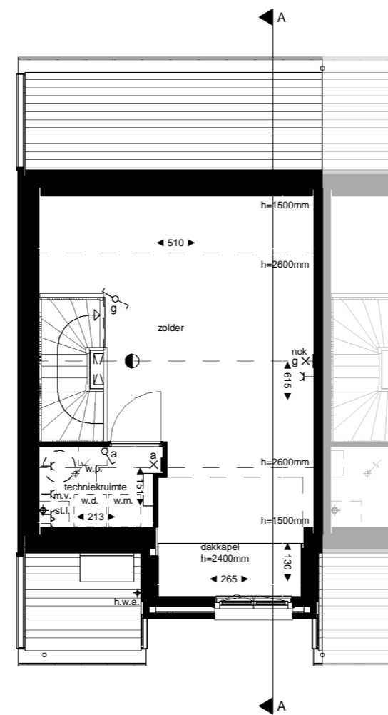
Zolder
