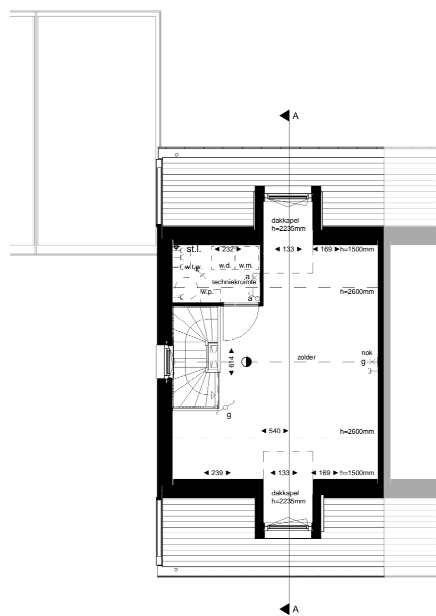
Zolder
